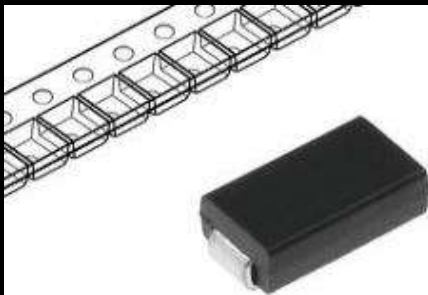
SMD 1N4001 M1 SMA M1 Diode rectifying SMD 50V 1A SMA
